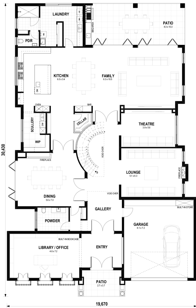
GROUND FLOOR 1:100
